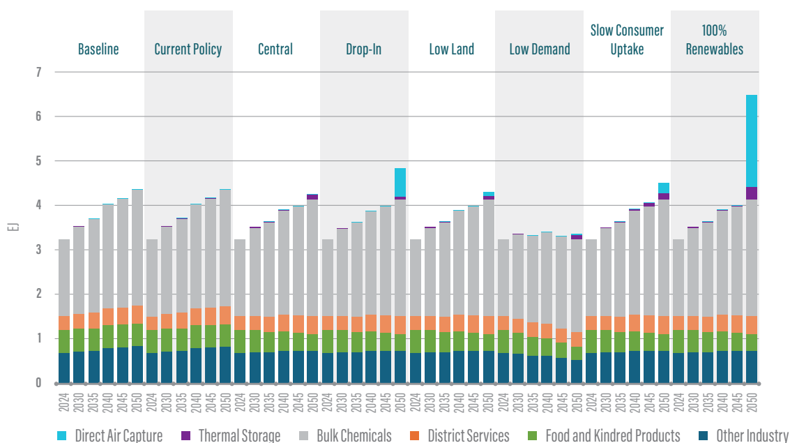
FIGURE 7. Uses of steam across scenarios
