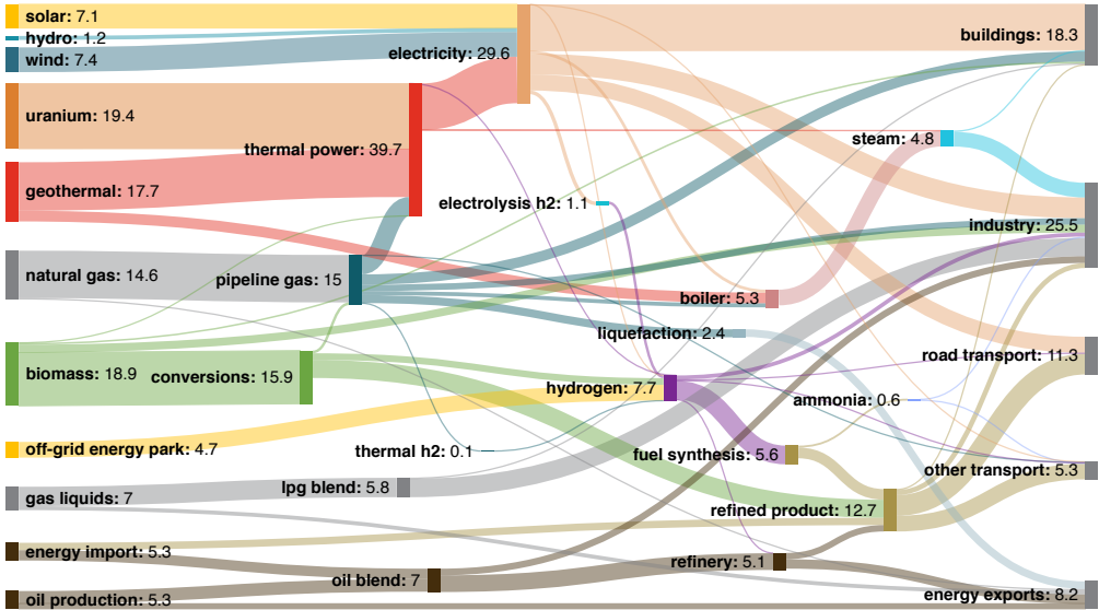
FIGURE 24. Sankey Diagram for 2050 Drop-In Scenario (Exajoules)
