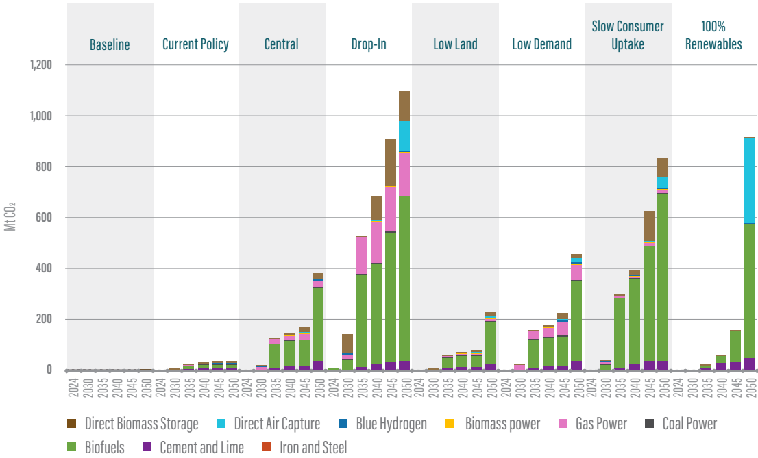
FIGURE 64. Carbon Capture Source
