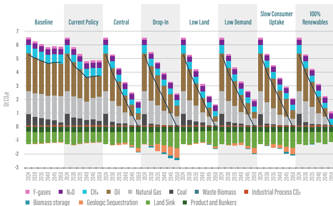
FIGURE 19. Greenhouse gas emissions by scenario (Gigatonnes)
