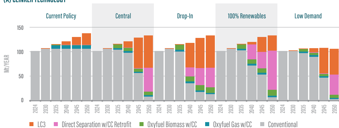
FIGURE 13. (Top) Clinker technology by type across scenarios (Bottom) Energy source for cement kiln heat
