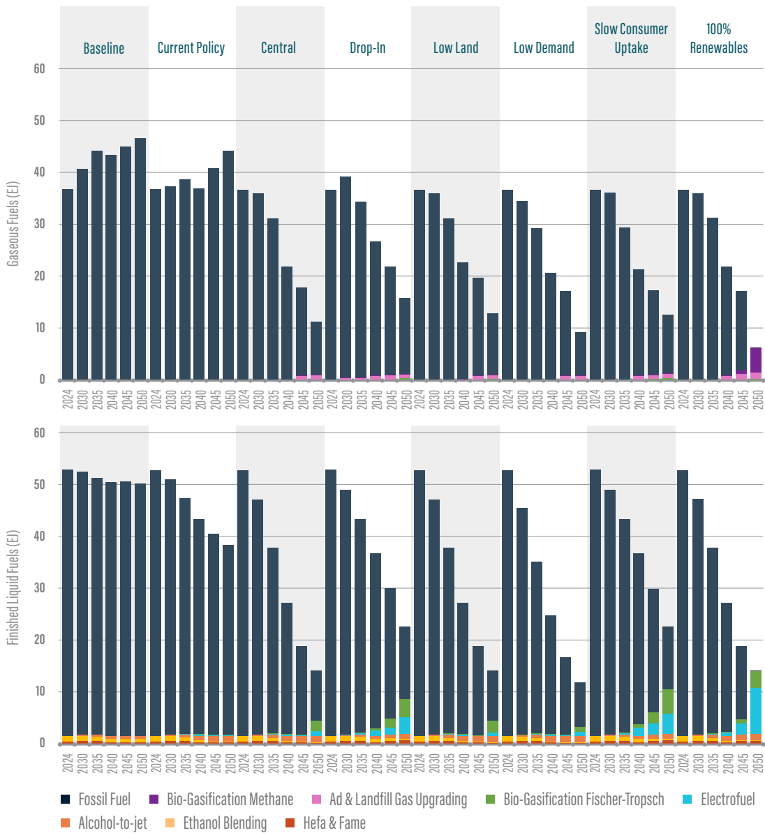
FIGURE 66. Hydrocarbon fuel supply
