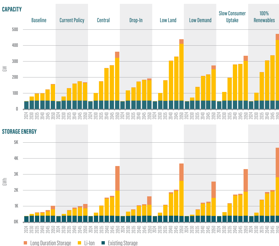
FIGURE 30. Electricity storage across scenarios. (Top) Power capacity (GW). (Bottom) Energy storage capacity (GWh)
