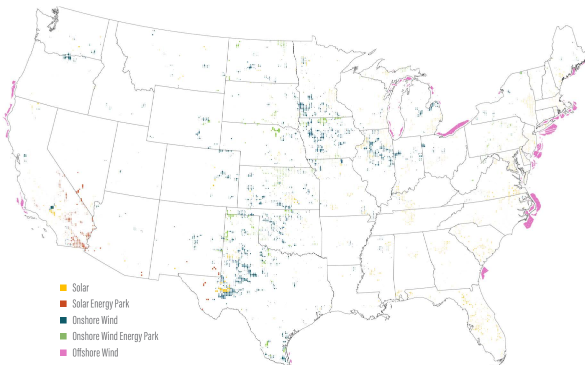
FIGURE 39. Downscaled wind and solar in 2050 for the Drop-In scenario
