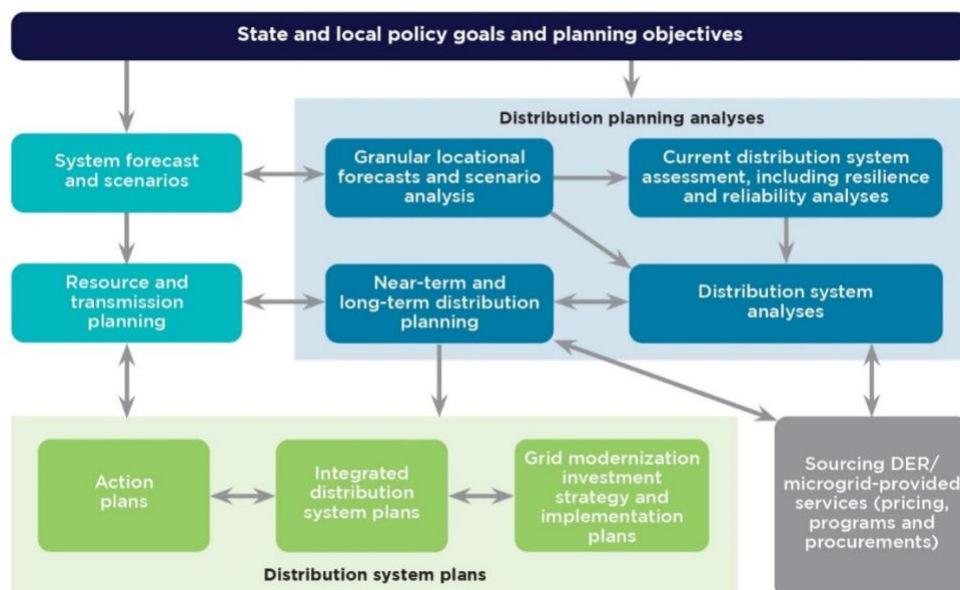
Figure 4. Flow Chart for Electric Distribution Planning
